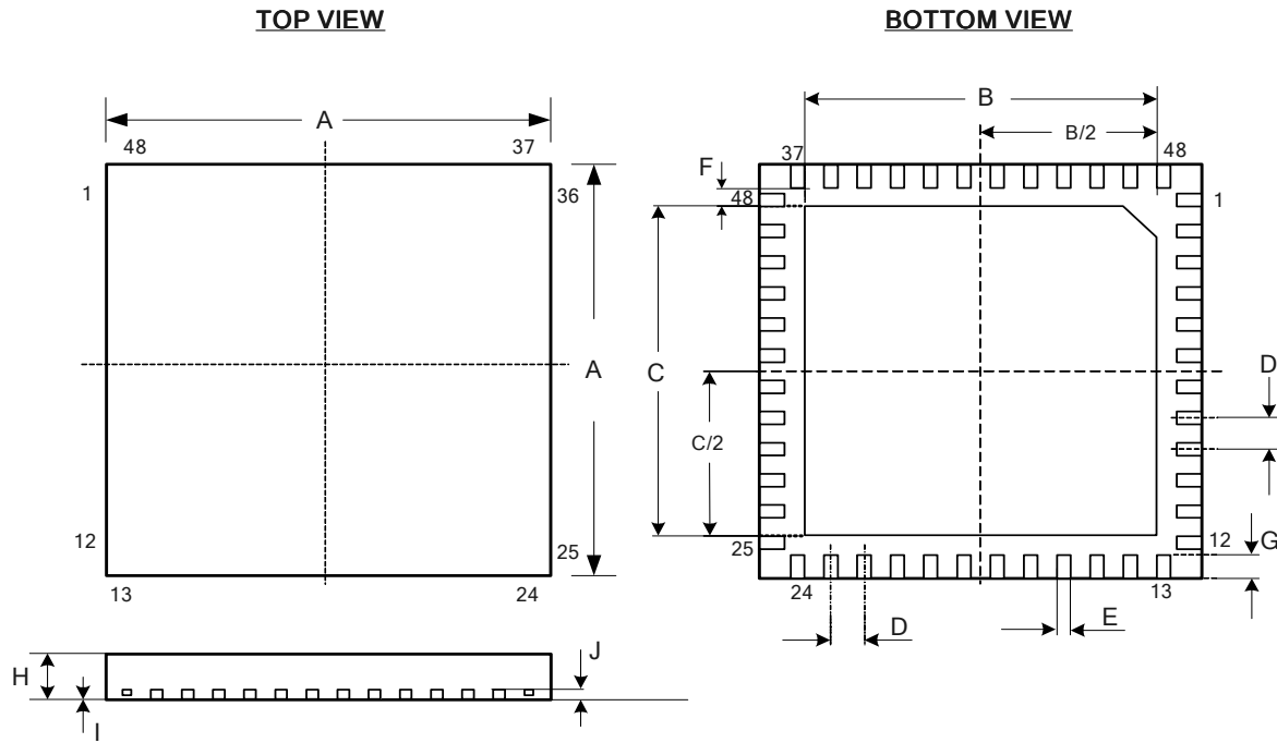
Figure 3: 48 Pin QFN Package
