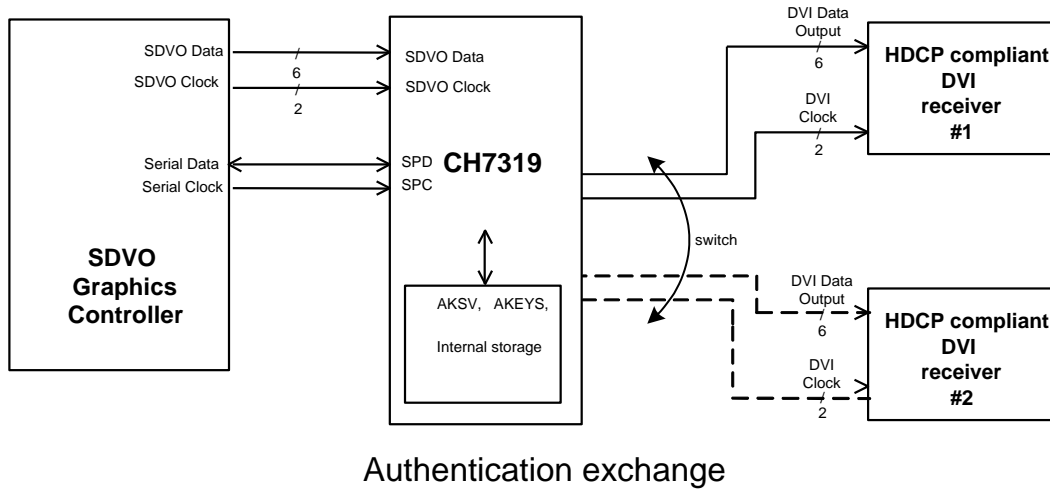
Authentication exchange Figure 3: Possible Connection Diagram for HDCP
