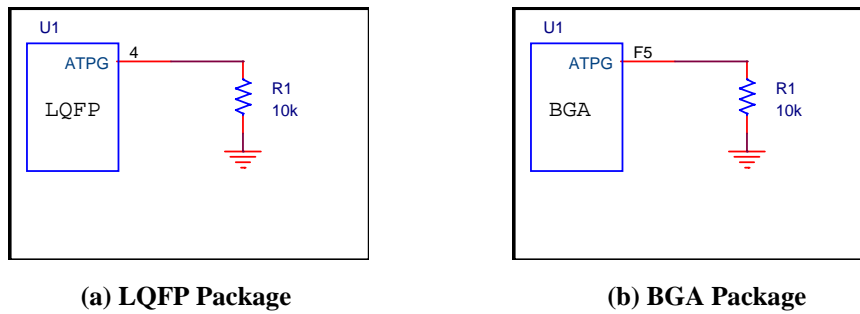
Figure 6: ATPG Pin
