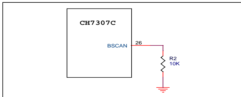
Figure 5: BSCAN strapping options
