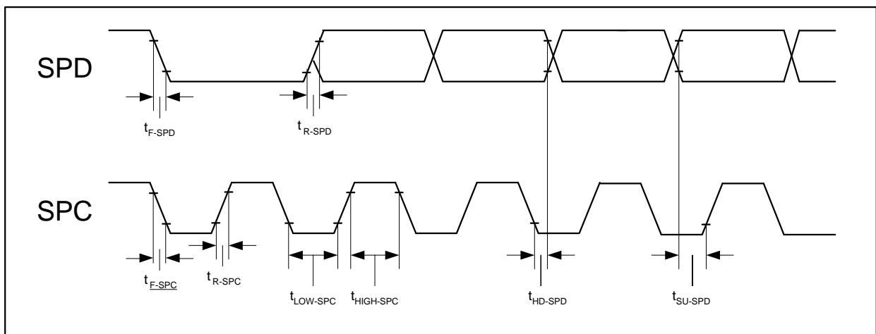
Figure 10: Serial Port Interface Timing
