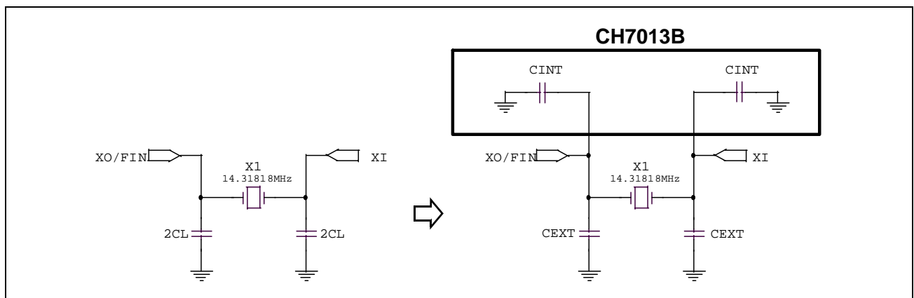
Figure 5: Reference Crystal
