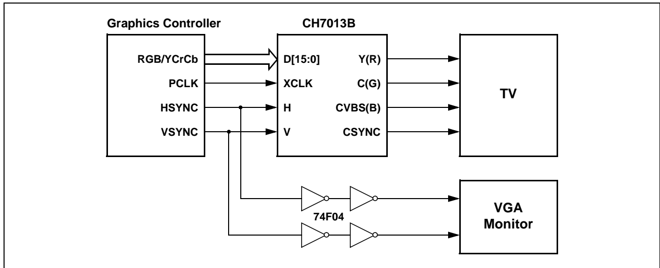
Figure 2: Sync Buffers
