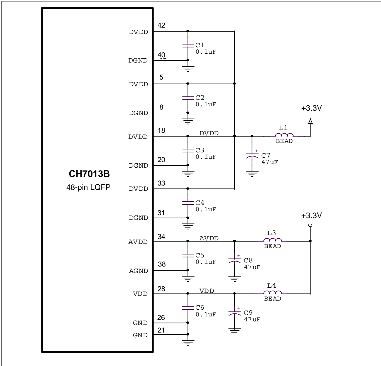
Figure 1: Power Supply Decoupling and Distribution
