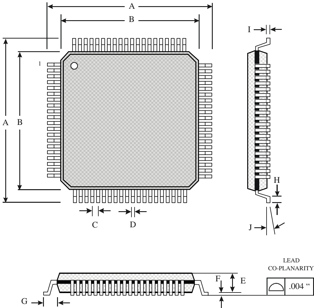
80 Pin LQFP Package
