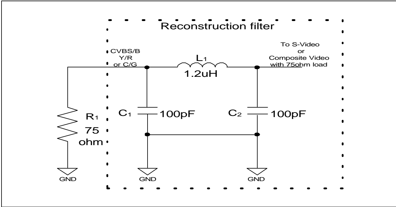
Figure 1: Reconstruction filter diagram
