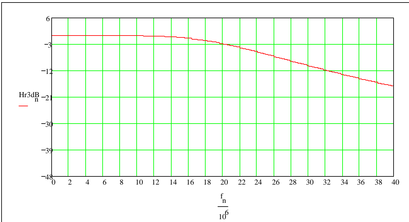
Figure 2: Frequency Response
